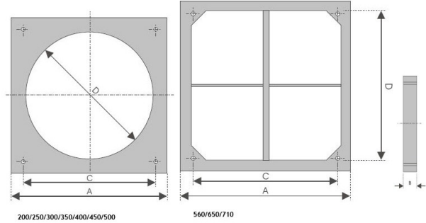
200/250/300/350/400/450/500
